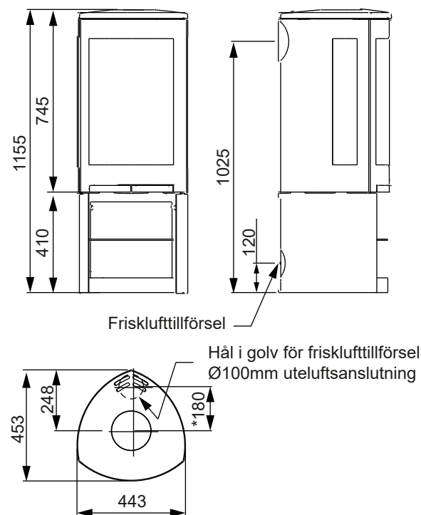
Jøtul F 371 Advance
